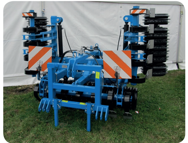
Châssis repliable
